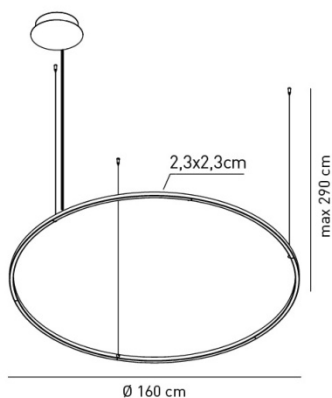
rosone standard / standard canopy
