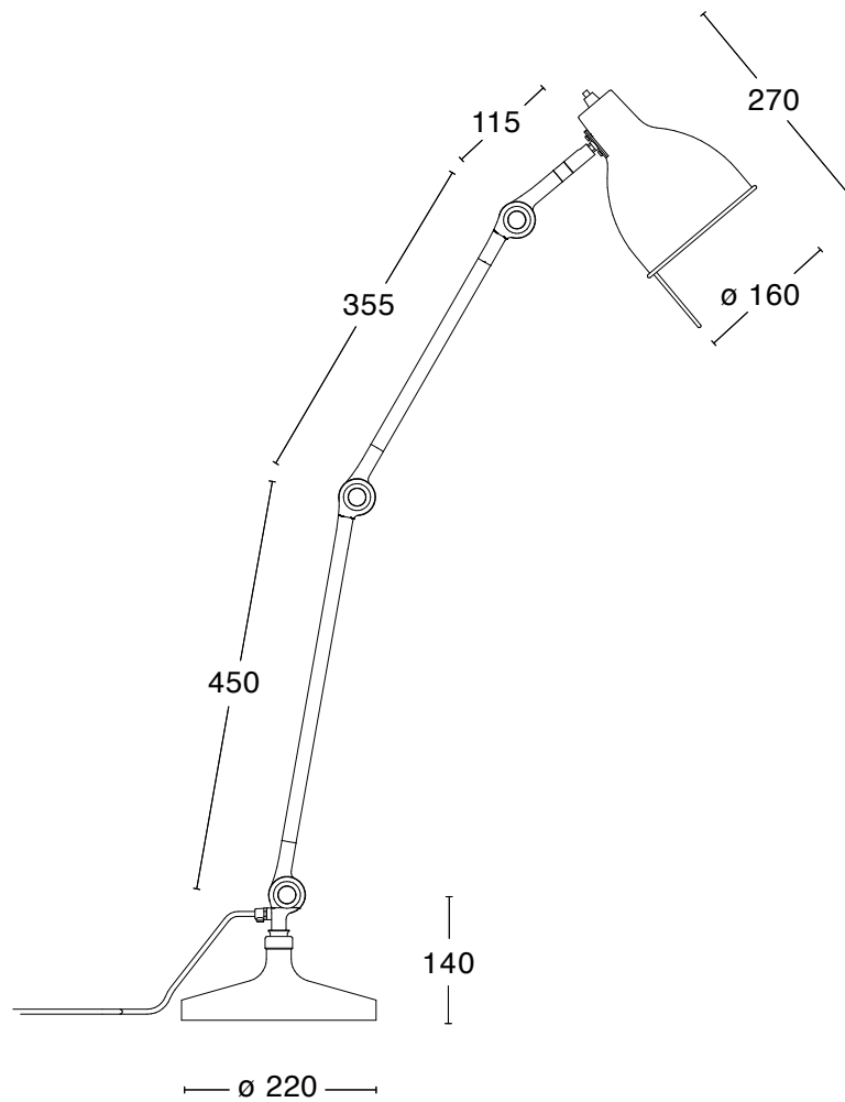
PJ60 LAMP FOOT
