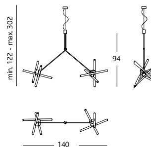
Double pending lamp
