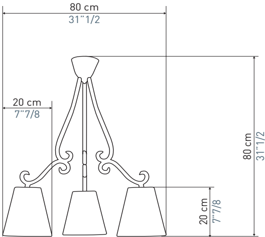
Suspension VOLUTE
