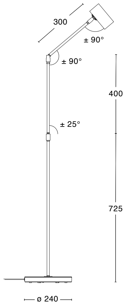
MINIPOINT FLOOR LAMP
