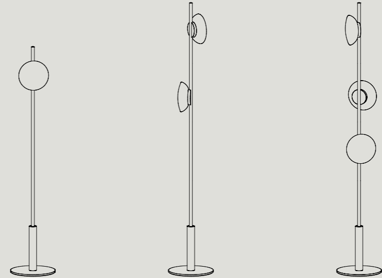
CF1 Ø 300 H 1560 Ø 11.8" H60.6" CF2 Ø 300 H 1840 Ø 11.8" H76.6" CF3 Ø 300 H 1840 Ø 11.8" H76.6"
