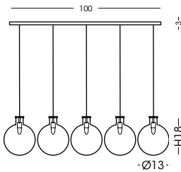
797.5L Binario a soffitto / Ceiling track vetro/glass Ø13 cm - cavo/cable 150 cm
