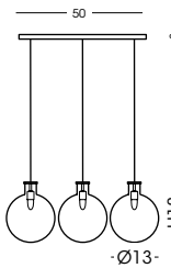
797.3L Binario a soffitto / Ceiling track vetro/glass Ø13 cm - cavo/cable 150 cm
