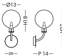
AP791.1L Applique / Wall lamp vetro/glass Ø13 cm - H20 cm
