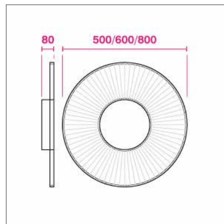
WALL MOUNTED CENTRAL BRACKET (MM)
