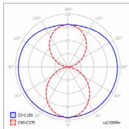
POLAR CURVE INTEGRATED LED (2700K)
