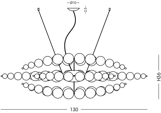
.8L Sospensione / Hanging lamp L130 cm - H36 cm - cavo/cable 150 cm 8 G9 x max 42W 230V CE IP20 1m
