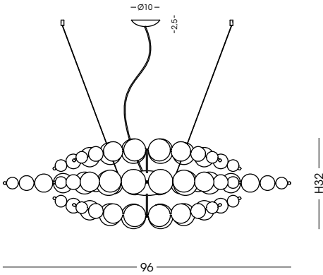
.6L Sospensione / Hanging lamp L96 cm - H32 cm - cavo/cable 150 cm 6 G9 x max 42W 230V CE IP20 1m
