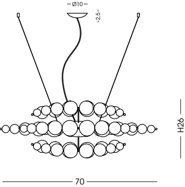
.4L Sospensione / Hanging lamp L70 cm - H26 cm - cavo/cable 150 cm 4 G9 x max 42W 230V CE IP20 1m
