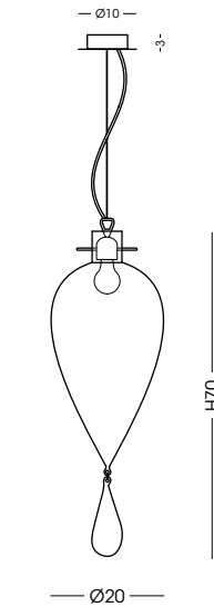
GIG803.1L Sospensione / Hanging lamp vetro/glass Ø20 cm - cavo/cable 150 cm 1 E27 x max 70W 220-240V CE IP20 1m
