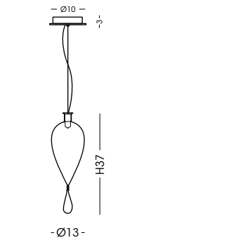
803.1L Sospensione / Hanging lamp vetro/glass Ø13 cm - cavo/cable 150 cm 1 G9 x max 42W 230V CE IP20 1m
