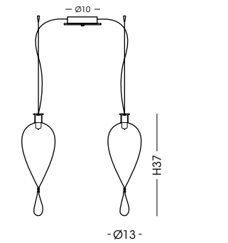
803.2L Sospensione / Hanging lamp vetro/glass Ø13 cm - cavo/cable 250 cm 2 G9 x max 42W 230V CE IP20 1m
