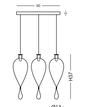
807.3L Binario a soffitto / Ceiling track vetro/glass Ø13 cm - cavo/cable 150 cm 3 G9 x max 42W 230V CE IP20 1m
