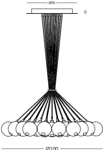
1292.37L Plafoniera / Ceiling lamp vetro/glass Ø14 cm - Cavo/Cable 250 cm 37 G9 x max 33W 230V CE IP20 1m
