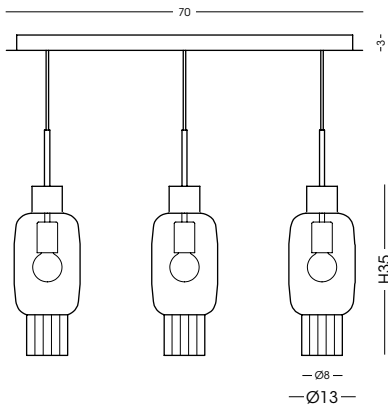
1367.3L Binario a soffitto / Ceiling track vetro/glass Ø13 cm - cavo/cable 150 cm 3 E27 x max 42W 220-240V CE IP20 1m
