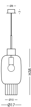
GIG1363.1L Sospensione / Hanging lamp vetro/glass Ø17 cm - cavo/cable 150 cm 1 E27 x max 70W 220-240V CE IP20 1m
