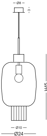
XXL1363.1L Sospensione / Hanging lamp vetro/glass Ø24 cm - cavo/cable 150 cm 1 E27 x max 70W 220-240V CE IP20 1m
