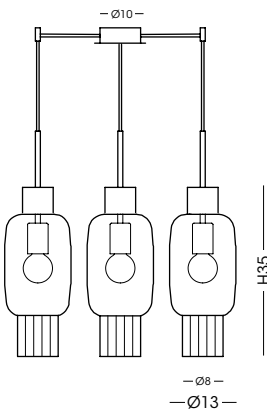
1363.3L Sospensione / Hanging lamp vetro/glass Ø13 cm - cavo/cable 250 cm 3 E27 x max 42W 220-240V CE IP20 1m
