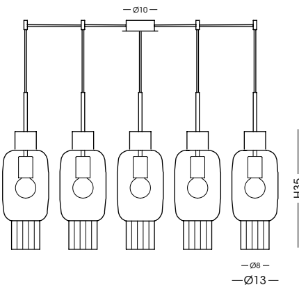
1363.5L Sospensione / Hanging lamp vetro/glass Ø13 cm - cavo/cable 250 cm 5 E27 x max 42W 220-240V CE IP20 1m
