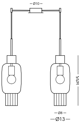
1363.2L Sospensione / Hanging lamp vetro/glass Ø13 cm - cavo/cable 250 cm 2 E27 x max 42W 220-240V CE IP20 1m
