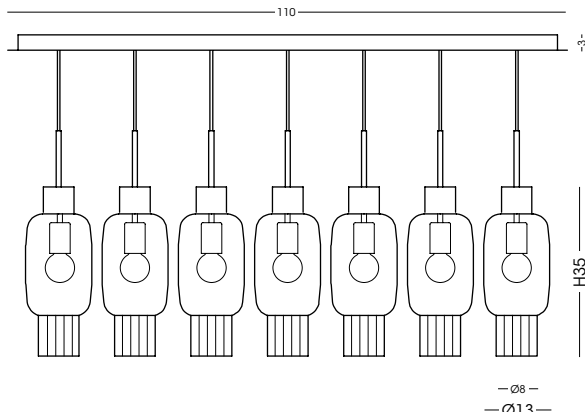
1367.7L Binario a soffitto / Ceiling track vetro/glass Ø13 cm - cavo/cable 150 cm 7 E27 x max 42W 220-240V CE IP20 1m
