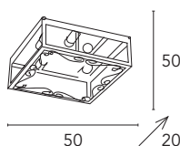
Vittoria 1390/PL50Q 4 x max 60W E27 230V
