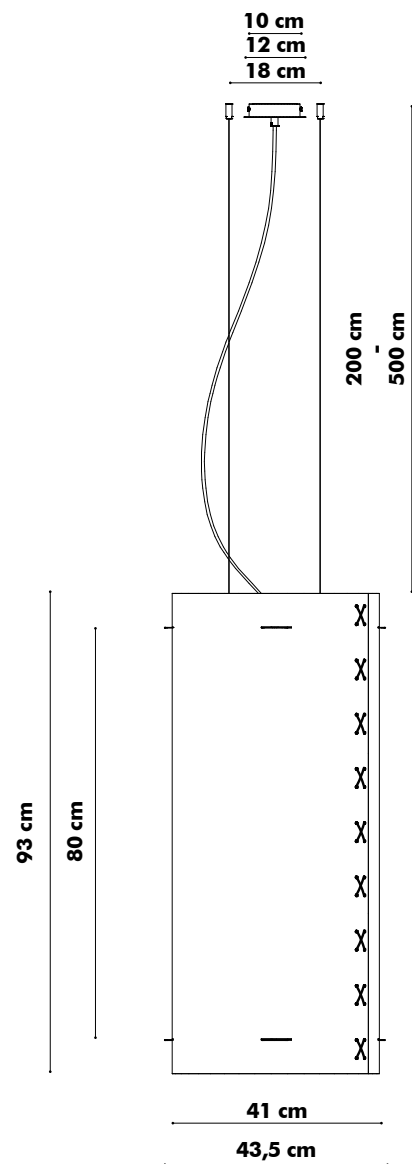
BuzziLight Alhambra | Royal XL High
