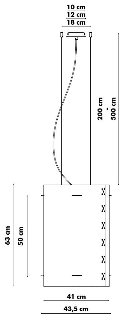
BuzziLight Alhambra | Royal XL Low
