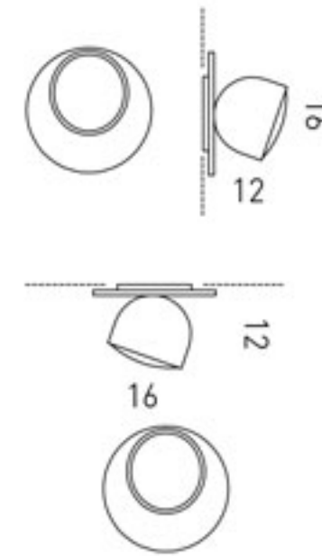
LS 4/310 8,5W LED 3000K 620 lumen CE IP20
