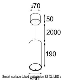
Smart surface tubed 82 large LED GI white struc
