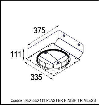
Conbox 375X335X111 PLASTER FINISH TRIMLESS
