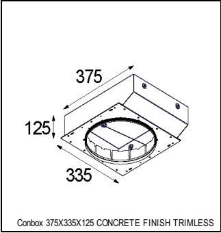
Conbox 375X335X125 CONCRETE FINISH TRIMLESS
