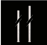
Code: 248 Pole with Base and Access Door With Terminal Block 4x1,5-16mmq ø76 mm H 3500 mm .6 grey .3 anthracite
