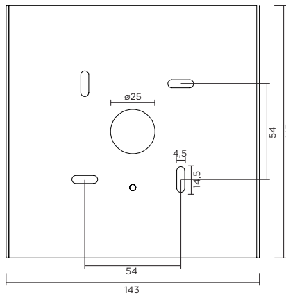
ceiling base dimensions
