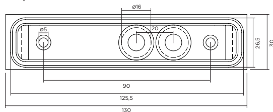
back plate dimensions
