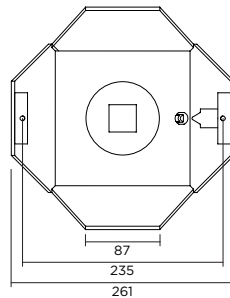
bracket dimensions - ALICE 2.0
