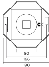
bracket dimensions - ALICE 1.0
