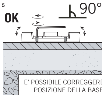
THE FIXING BASE POSITION IT'S ADJUSTABLE
