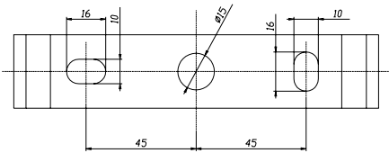
MINIFOCUS 149x30 mm
