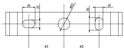
MINIFOCUS 149x30 mm
