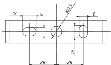
MICROFOCUS 98x22 mm
