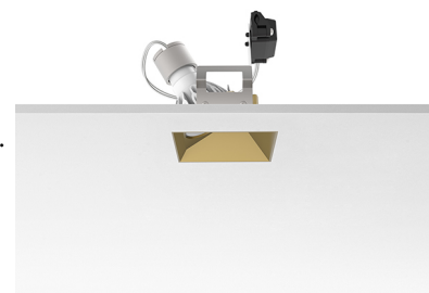
Kap 80 Square Wall-Washer designed by FLOS Architectural
