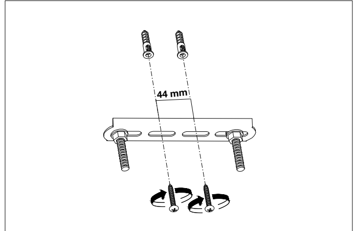
2. Fix the ceiling plate to the ceiling by using mounting plugs and screws suitable for your ceiling type.
