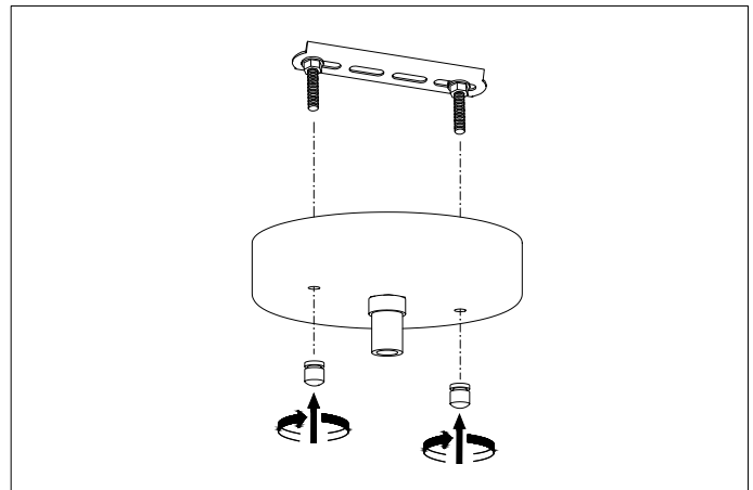
4. Slide the canopy over the ceiling plate and fix it with the two nuts.
