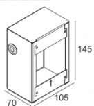
CONCRETE BOX 186 270 11 186
