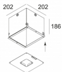
CONCRETE BOX 161 270 11 161
