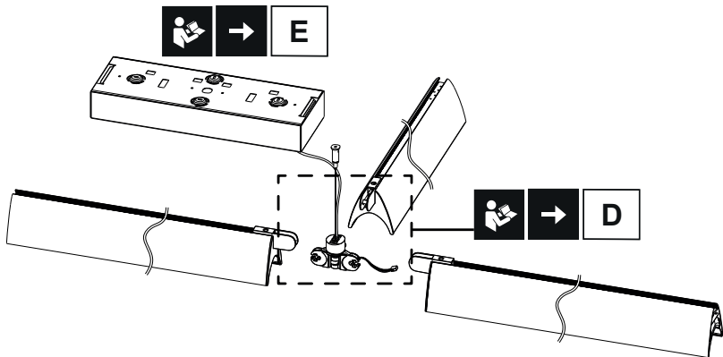
Joint system with electrical alimentation
