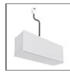
150W Ceiling power supply kit - 321x91x111H - 230VAC-48VDC IP20 - Dimmable DALI - Black AQ17704
