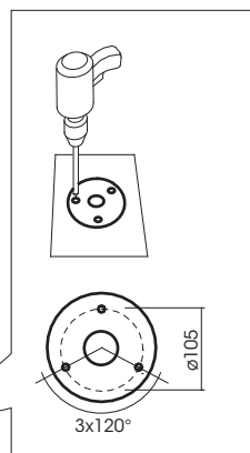
OPTION 2: TASSELLO - BOLTS
