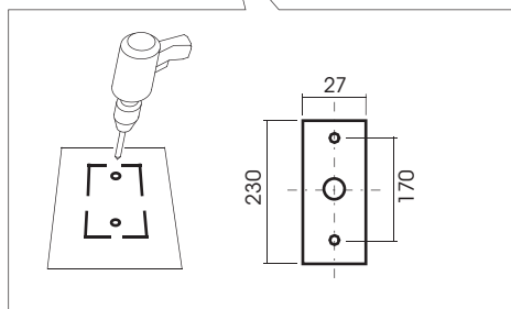
option 1: TASSELLO - BOLTS
