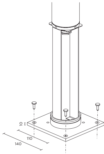
base plate dimensions
