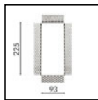
S.6074 MASK FOR PLASTER BOARD WALLS Hole 95 x 225 mm
