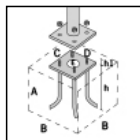
S.2849 PLANTED ROOT for CYLINDRICAL POLE
