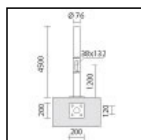
S.2845 Ø76mm CYLINDRICAL POLE WITH BASE
