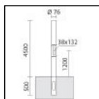
S.2844 Ø76mm CYLINDRICAL POLE TO BE BURIED
