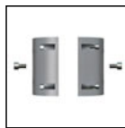
S.1013 FLANGE FOR POLE INSTALLATION Ø 120mm Flange in die-cast aluminium suitable only for Ø 120 mm poles. The flange can be used for maximum 2 projectors, one for each side.
