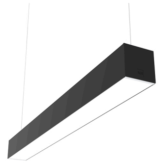
In-Finity 100 Suspension Down 4000K Micro-Prismatic Diffuser Dali
