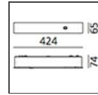
Kit driver linear and angular connector - 1M. + 1M. Occupies 1 DALI destination M305721
