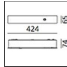
Kit driver linear and angular connector - 2M. + 2M. Occupies 2 DALI destinations M305921
