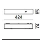
Kit driver linear and angular connector - 1M. + 2M. Occupies 2 DALI destinations M305821
