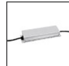
240W Bare power supply + plug 230VAC-48VDC IP20 - Undimmable (for dimmable version to be combined with "DALI-Selv interface") AQ18000
