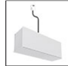
AQ25001 150W Ceiling power supply kit - 321x91x111H - 230VAC-48VDC IP20 - Dimmable DALI - White AQ17701
