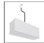
150W Ceiling power supply kit - 321x91x111H - 230VAC-48VDC IP20 - Dimmable DALI - Black AQ17704
