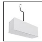
240W Ceiling power supply kit - 321x91x111H - 230VAC-48VDC IP20 - Dimmable DALI - White AQ17201
